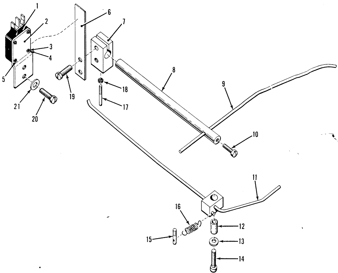
Figure 9. Film Buckle Switch and Levers.
