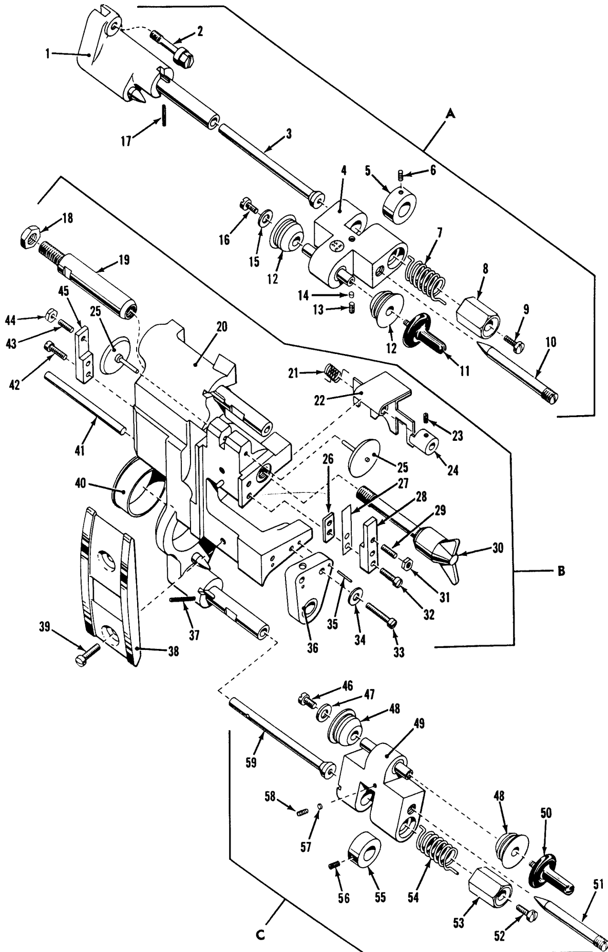
Figure 11. 35mm Film Gate and Pad Rollers.
