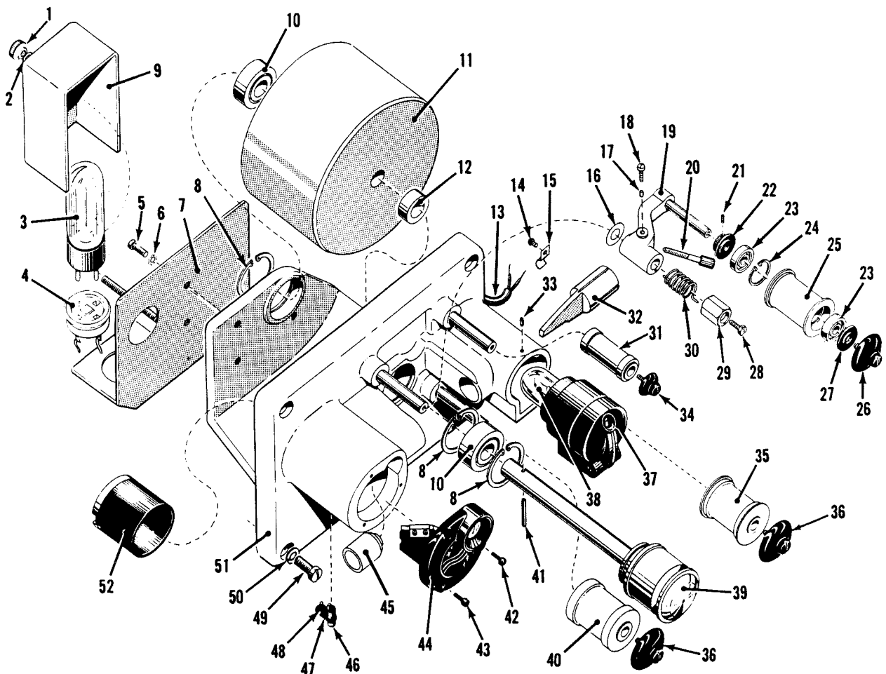
Figure 15. Optical Soundhead Cat. No. 3055
