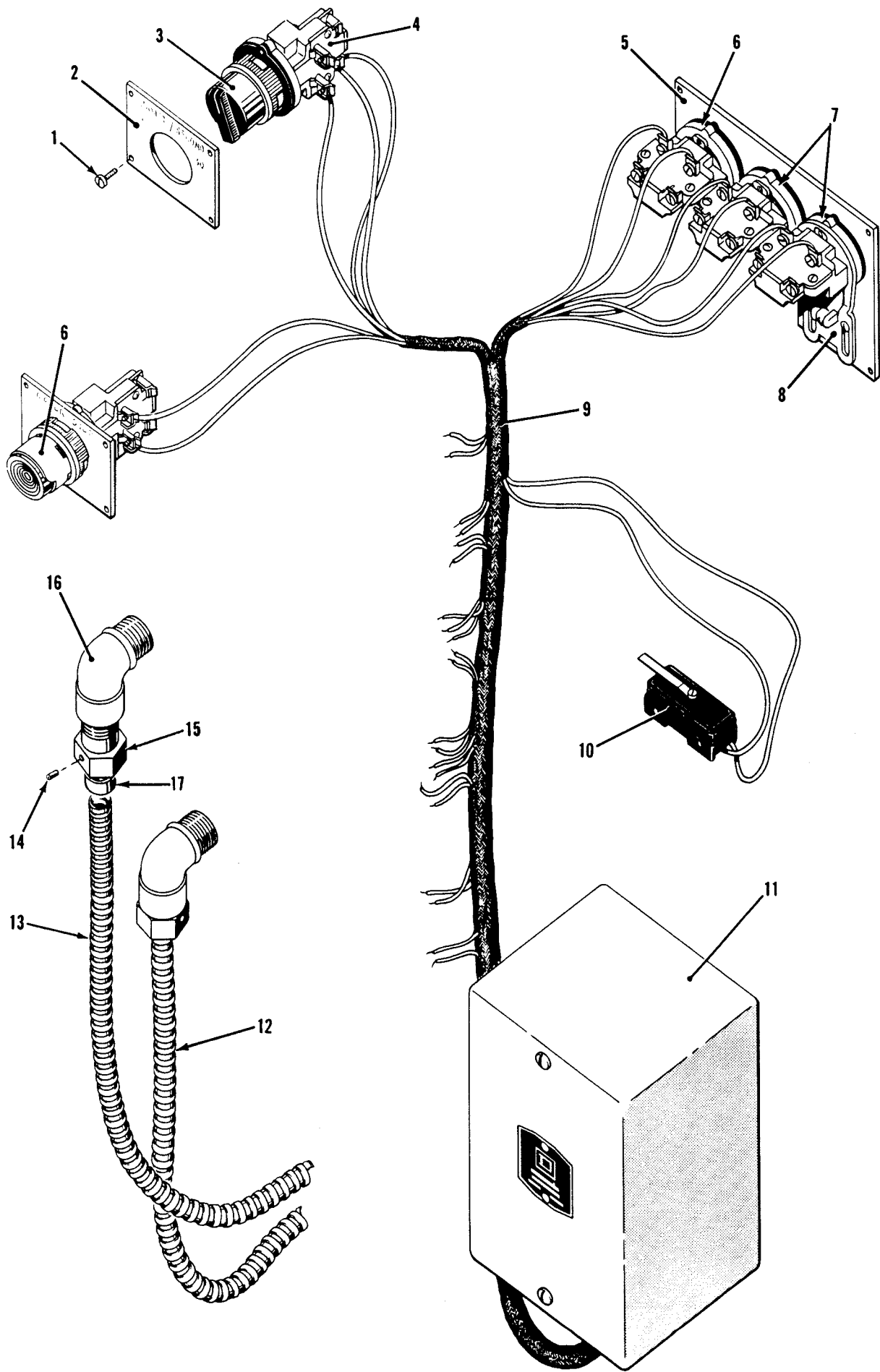
Figure 24. Electrical Components II.
