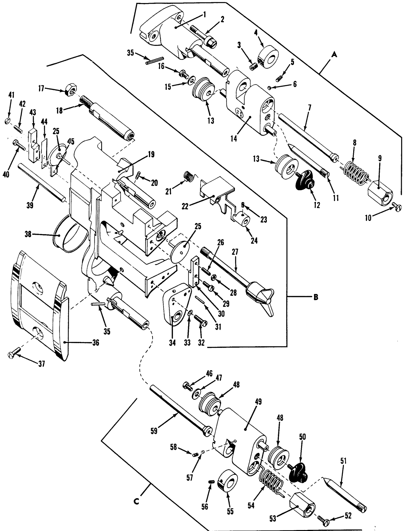
Figure 10. 70mm Film Gate and Pad Rollers.
