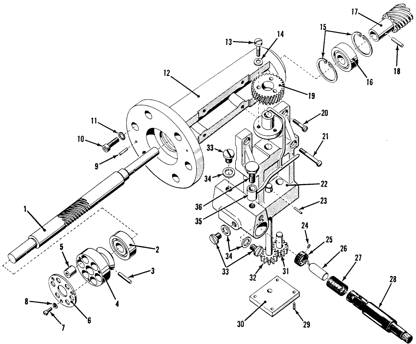
Figure 20. Oil Pump and Motor Drive Shaft.
