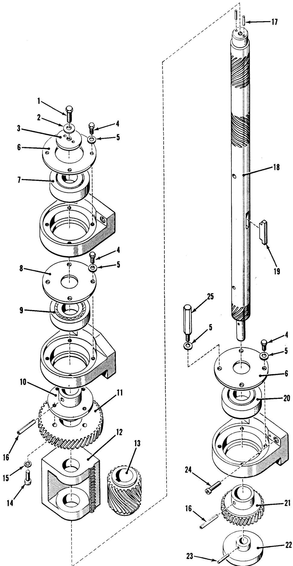
Figure 21. Main Shaft Assembly C1 750 50.
