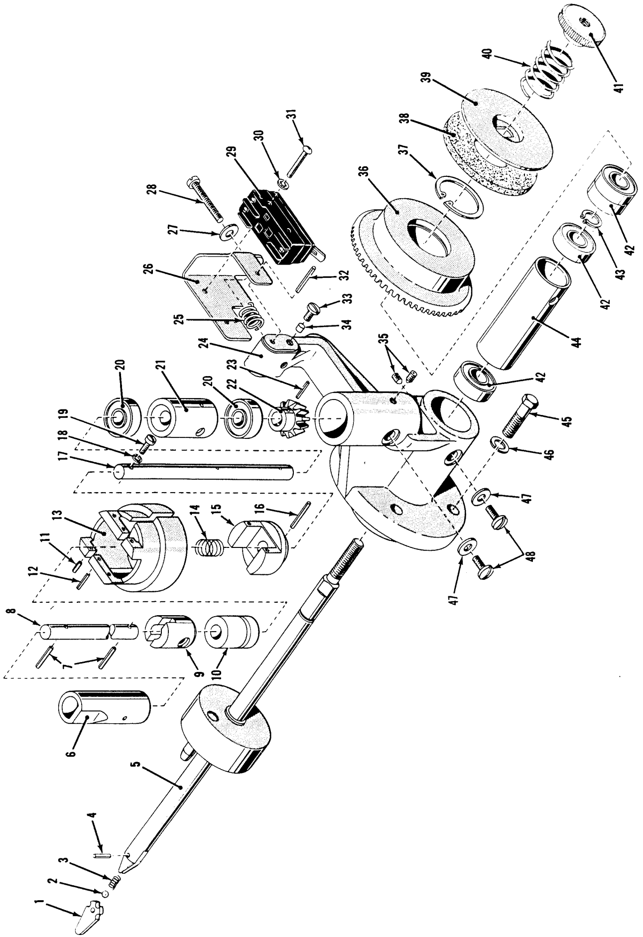
Figure 17. Take-Up Drive Assembly Cat. No. 3032.
