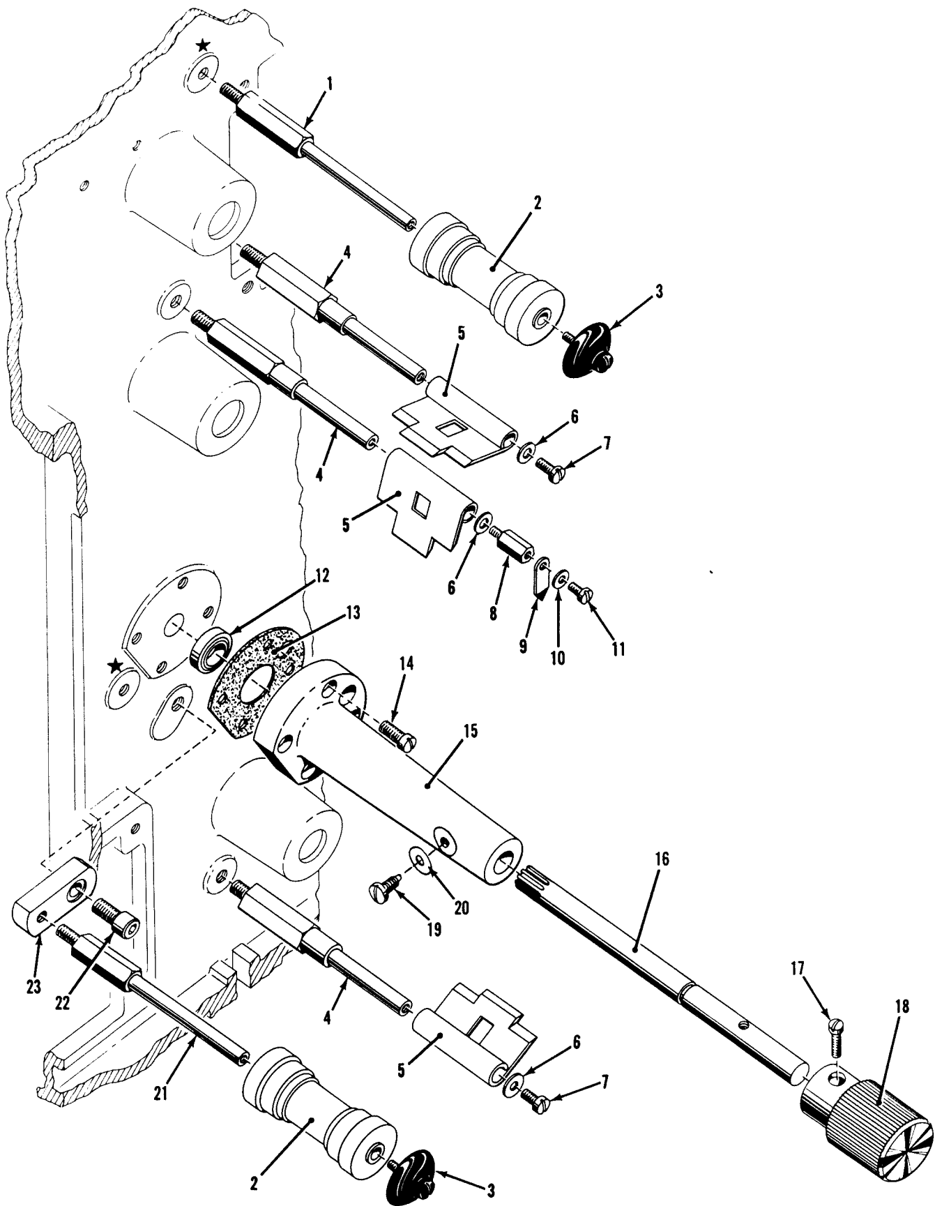
Figure 18. Guide Rollers, Film Strippers, and Framing Shaft Assembly.
