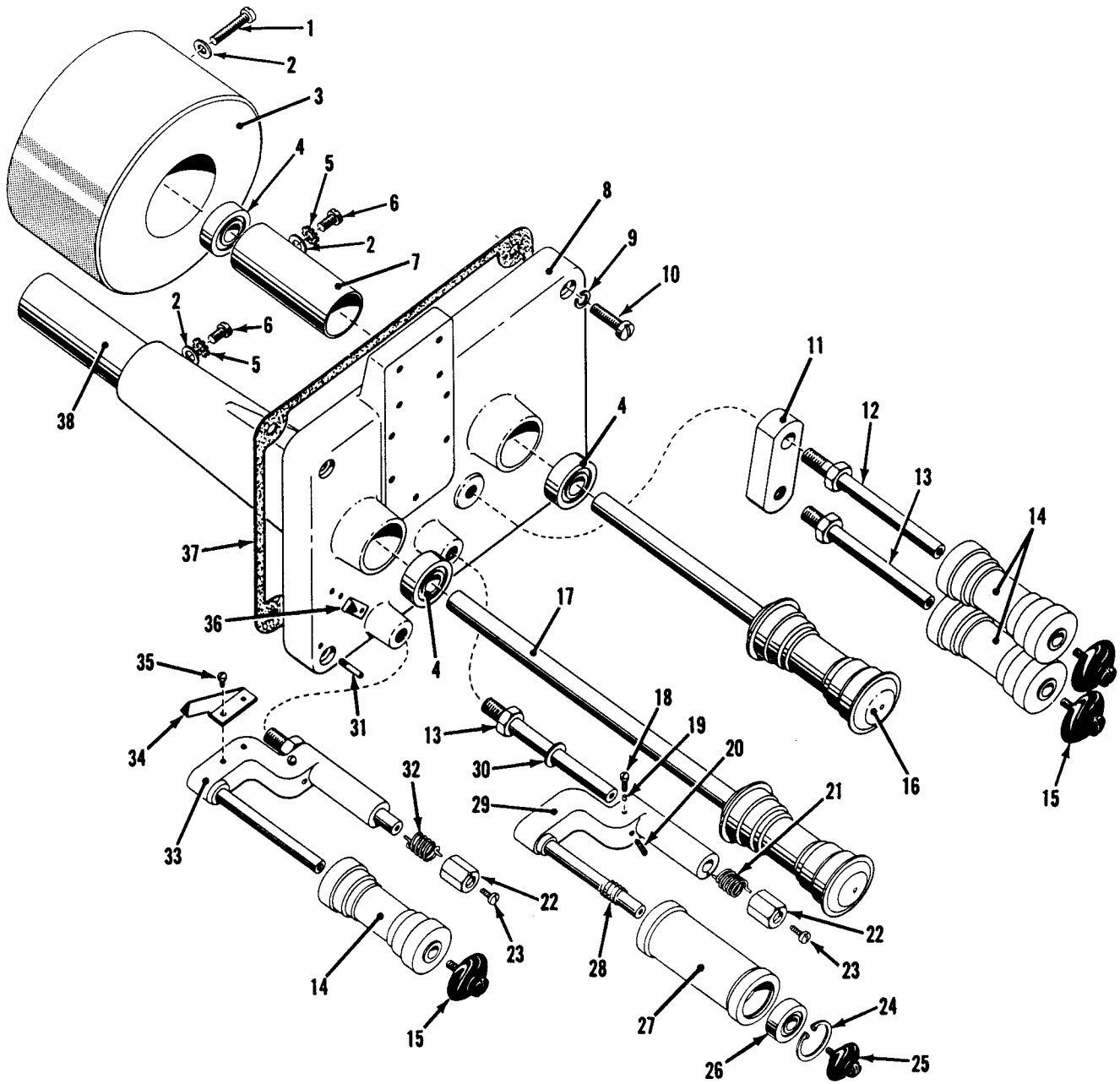
Figure 14. Magnetic Soundhead Cat. No. 3020.
