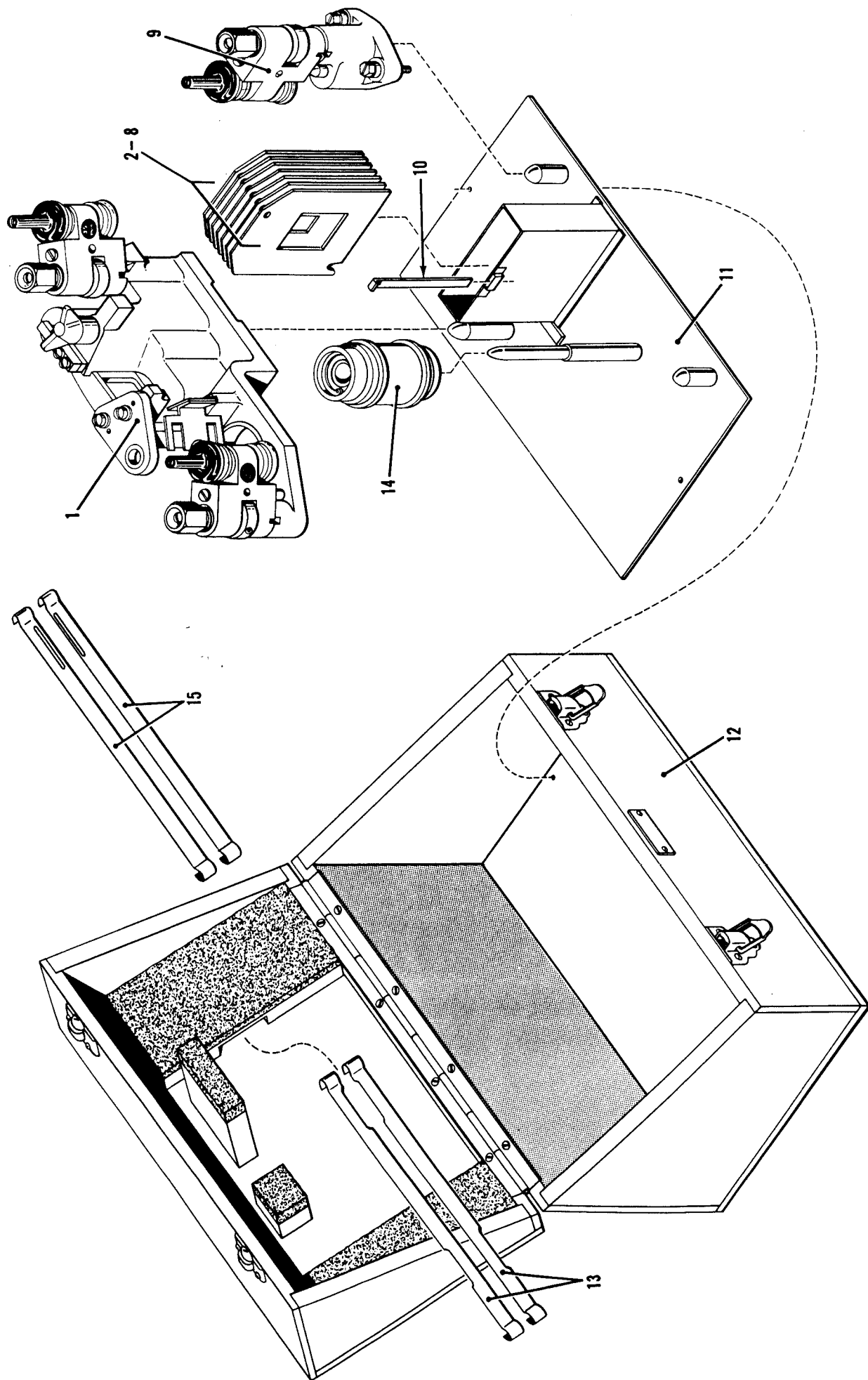
Figure 25. 35mm Conversion Parts and Chest Cat. No. 3018
