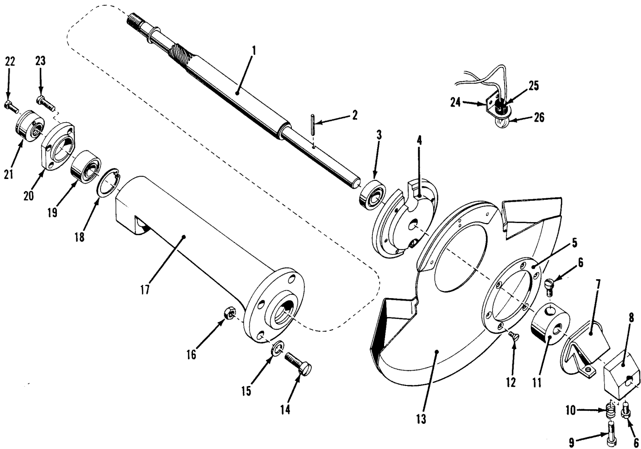
Figure 6. Shutter Shaft Assembly.
