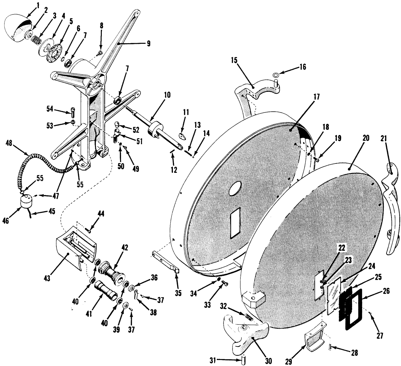
Figure 4. Upper Magazine and Fire Trap No. 3037
