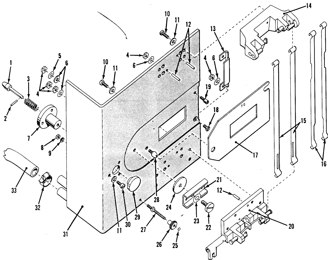
Figure 12. Cooling Plate C1 606 17.
