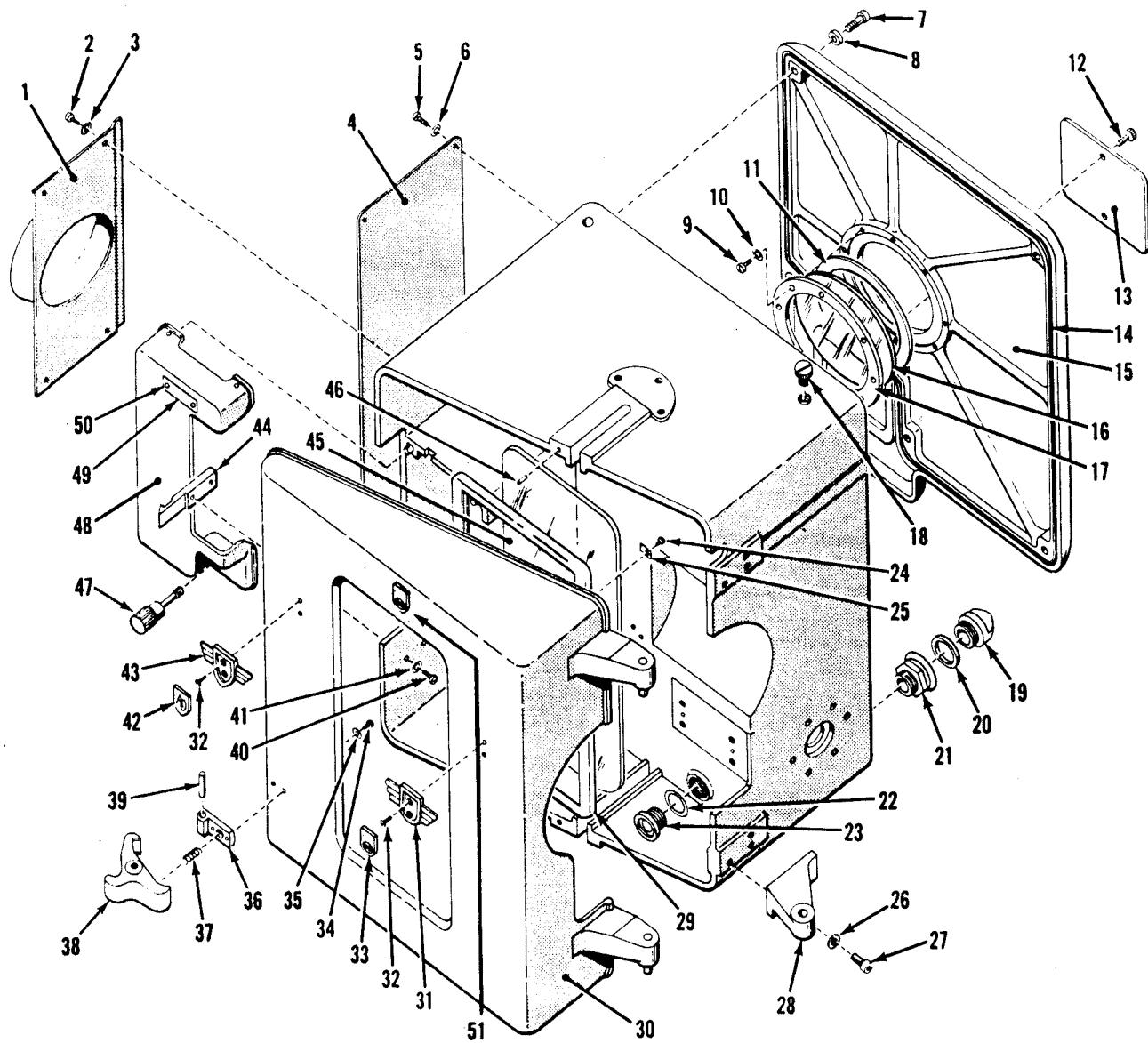
Figure 2. Projector Head - General.
