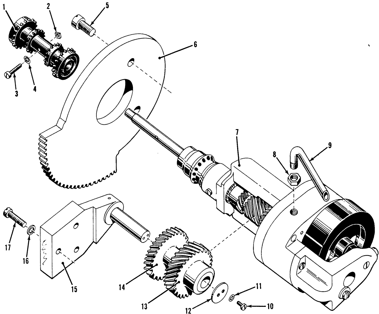
Figure 8. Intermittent Mechanism.
