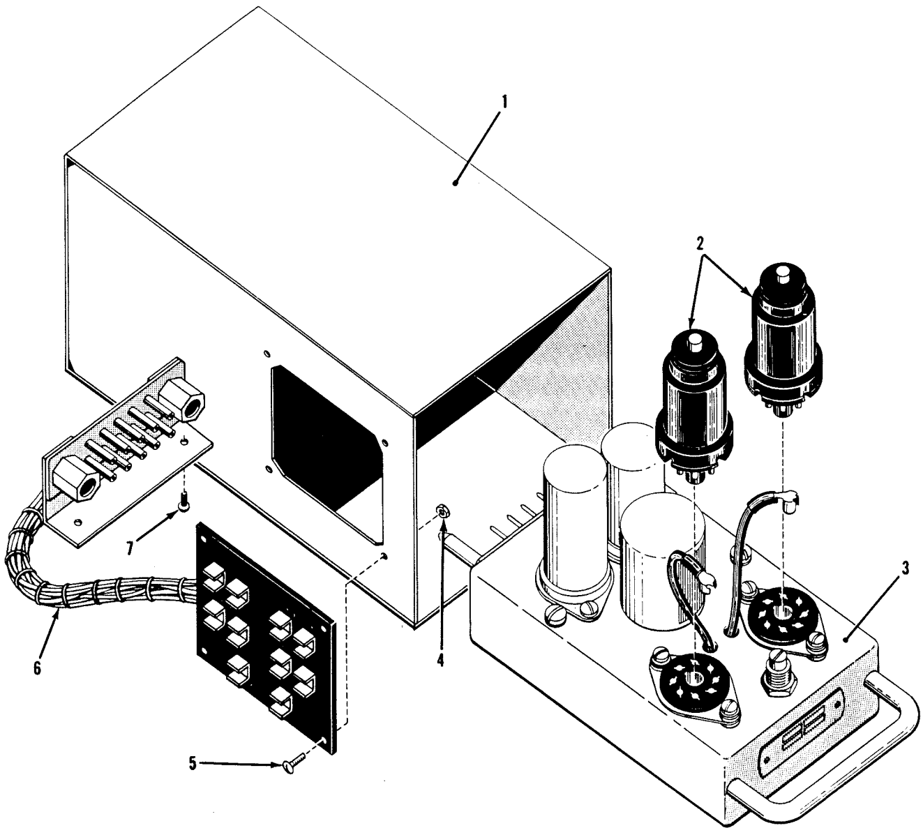
Figure 16. Optical Pre-amplifier.
