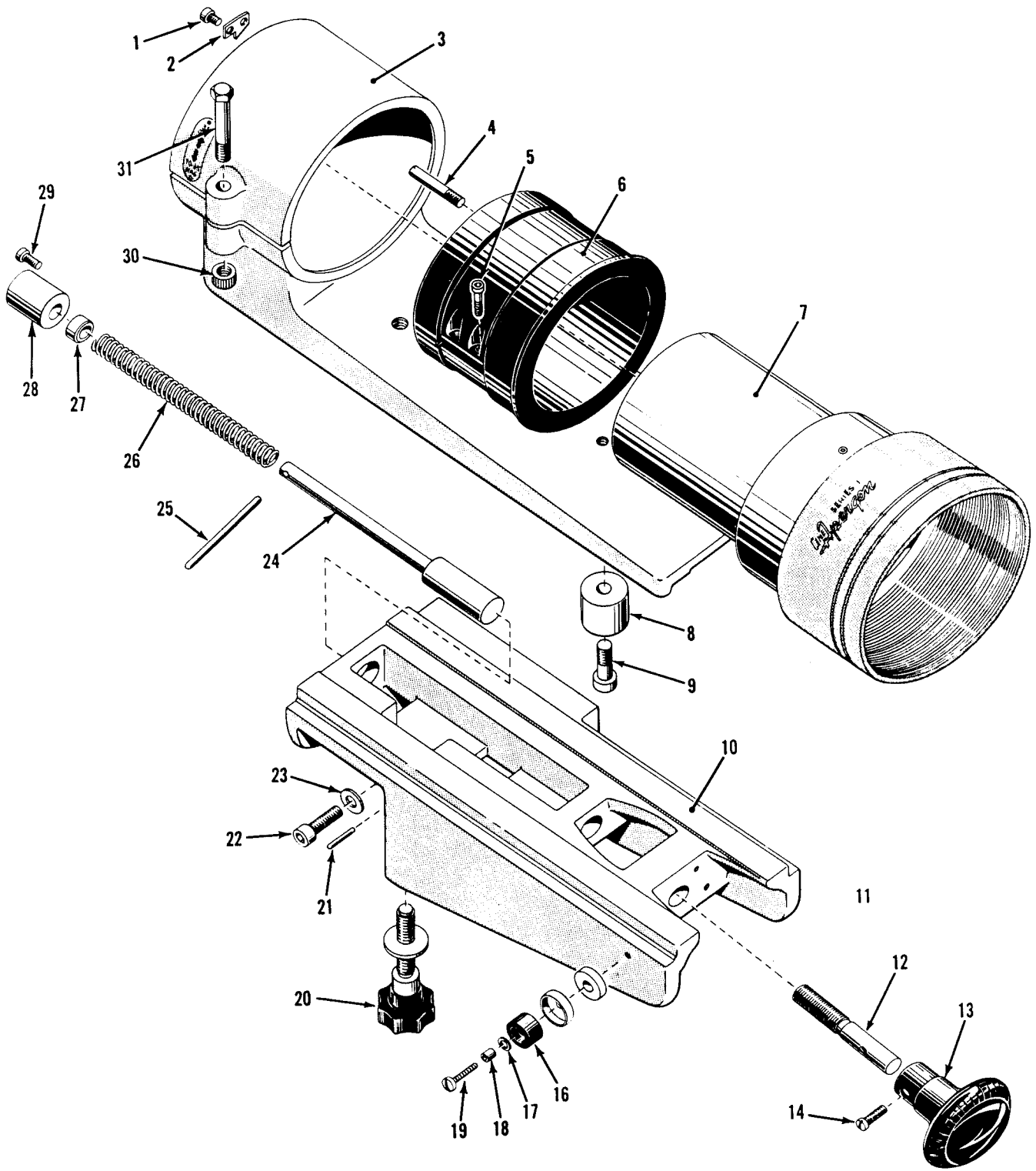
Figure 7. Lens Bracket Assembly.
