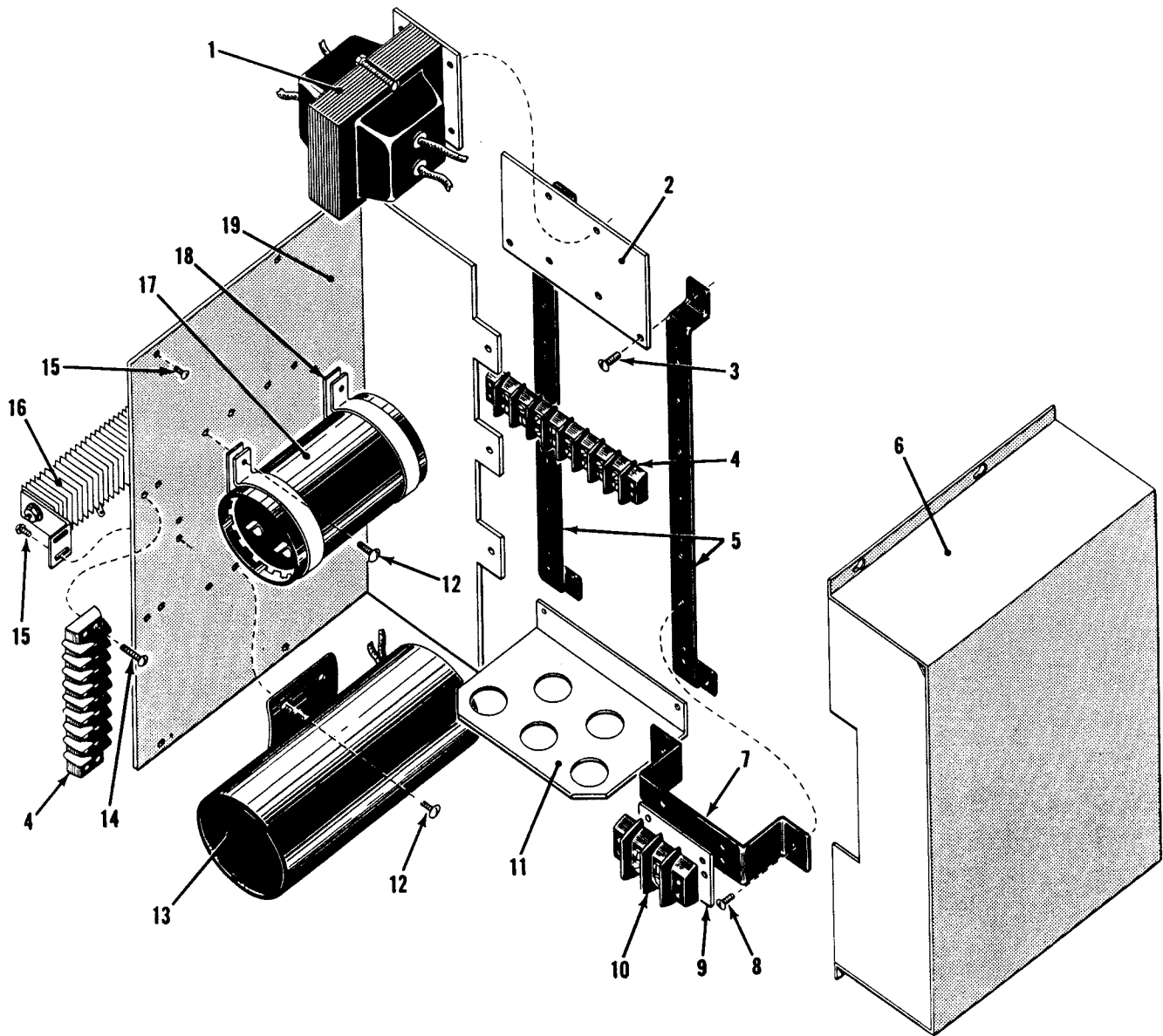
Figure 23. Electrical Components I.
