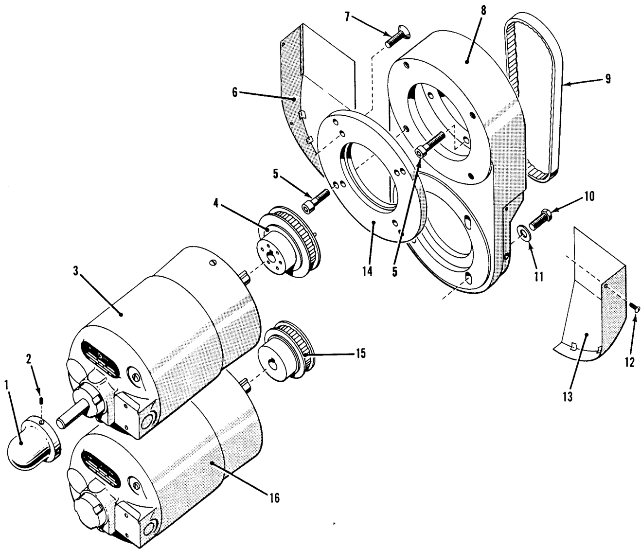
Figure 5. Motor Drive Assembly.
