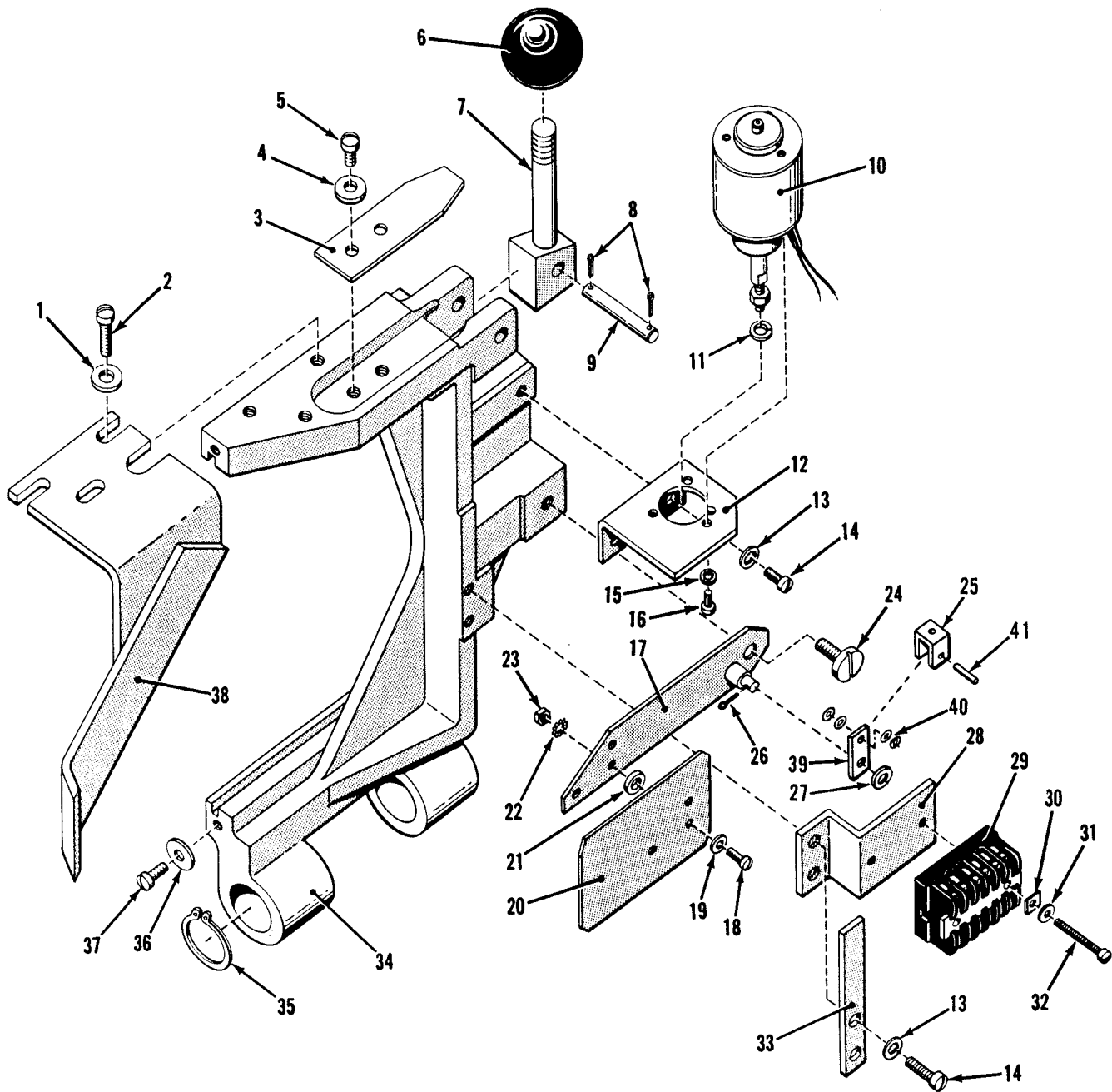
Figure 13. Cooling Plate Holder Assembly C1 703 65.
