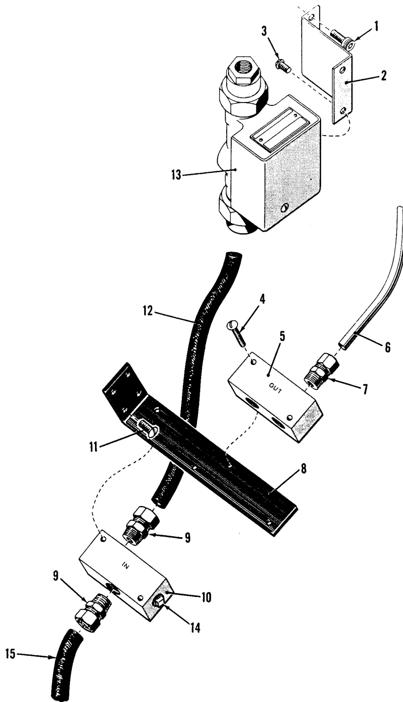
Figure 22. Water Manifolds and Flow Switch.
