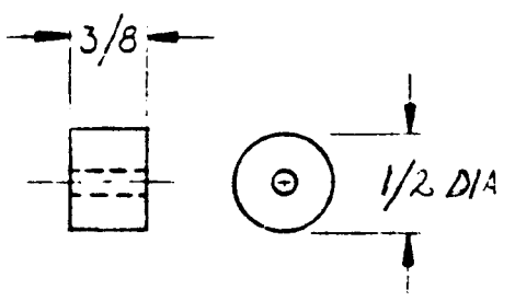
SWITCH ADJUSTMENT GAUGE
