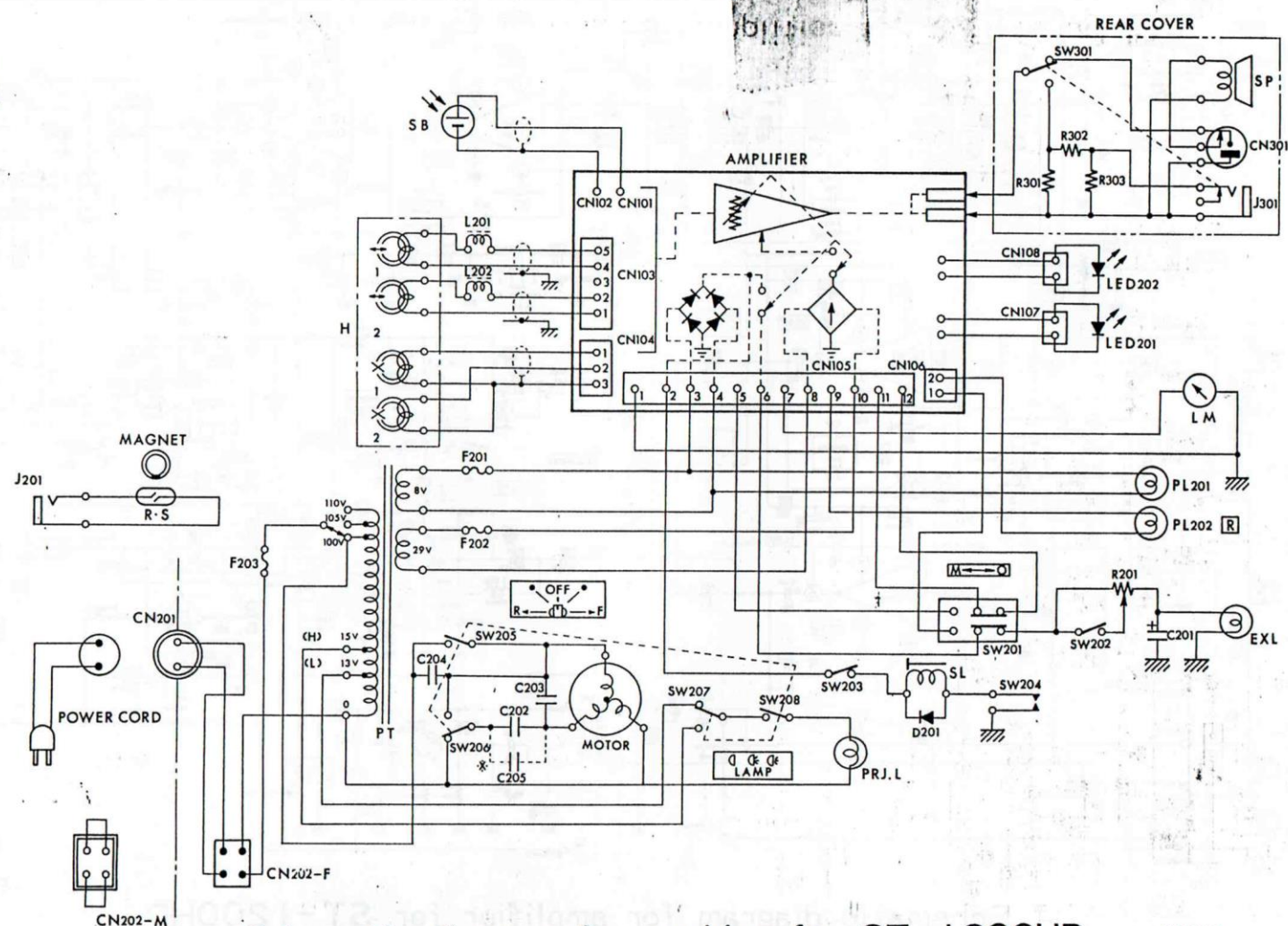
Schematic diagram for machine for ST-1200HD
